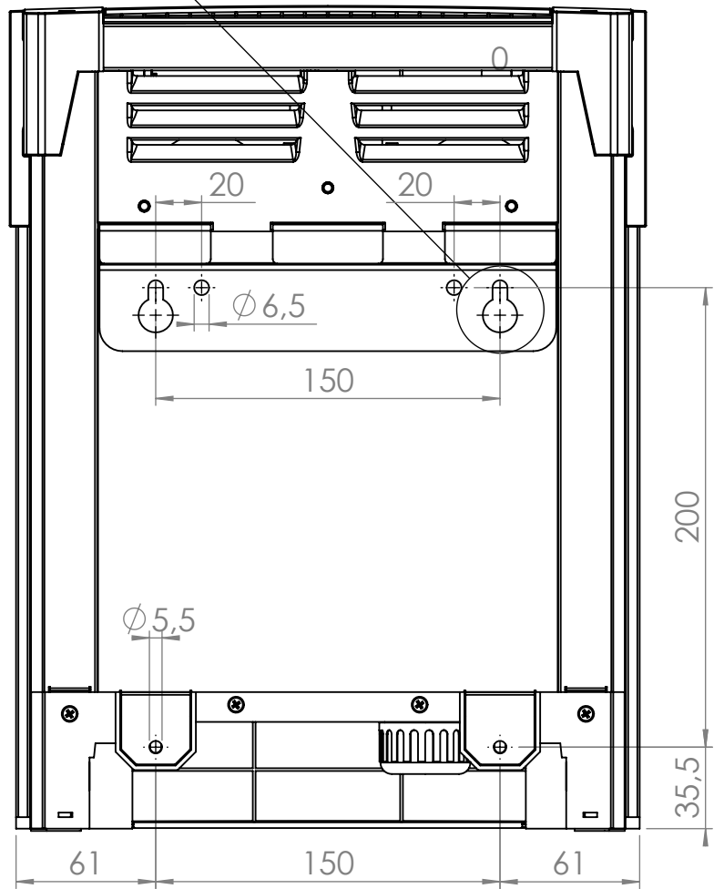
Backside: ChargeMaster II with mounting bracket.
